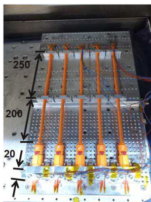
Figure 1: Vibration device (exemplary view)
