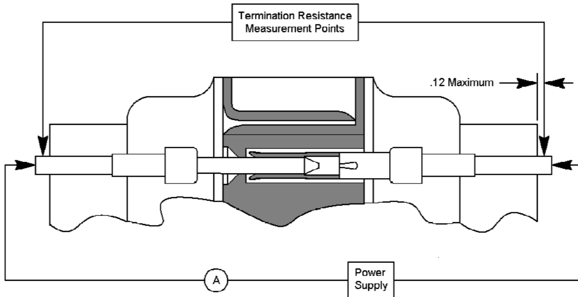
Figure 3 Termination Resistance Measurement Points
