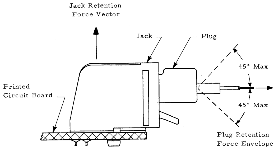
Figure 4 Plug and Jack Retention Forces
