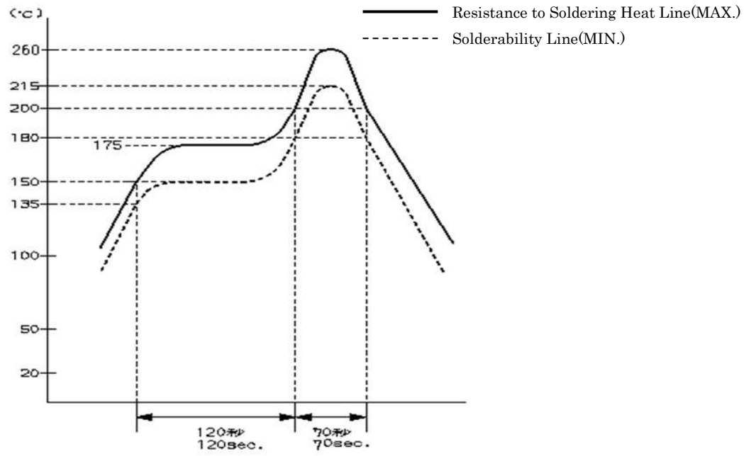
Fig. 3 Reflow Condition
