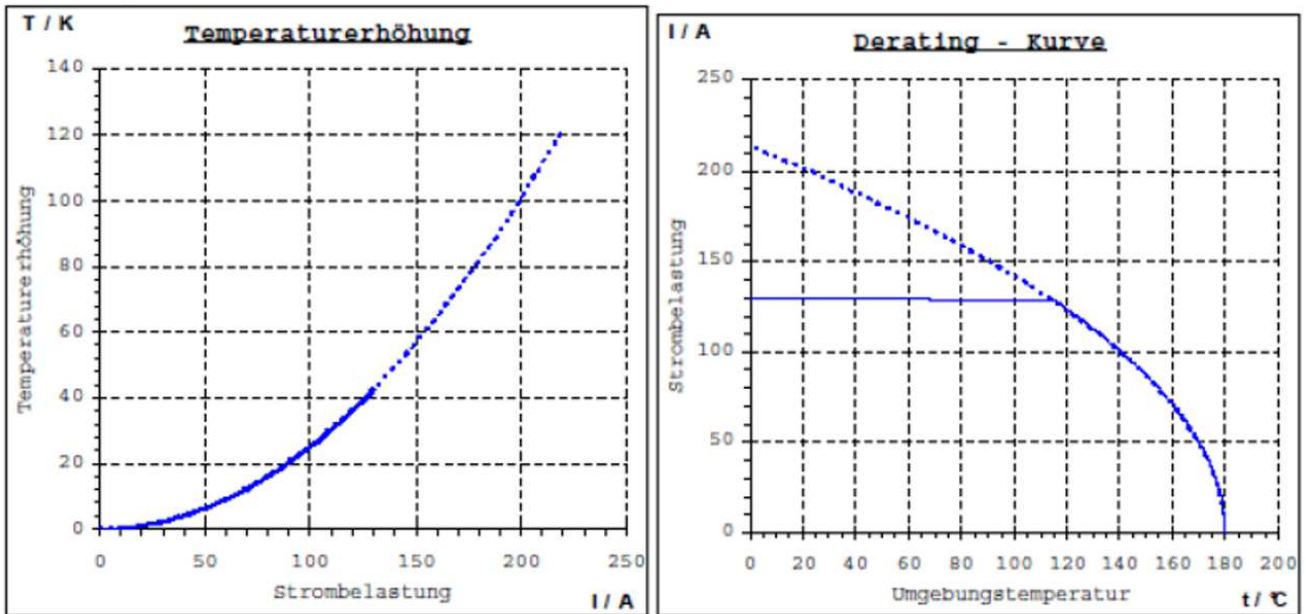
Figure1:Derating and temperature rise-1pos 25mm 2 Coroplast-Part-No.9-2611
