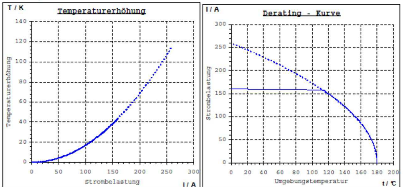
Figure2:Derating and temperature rise-1pos 35mm 2 Coroplast-Part-No.9-2611
