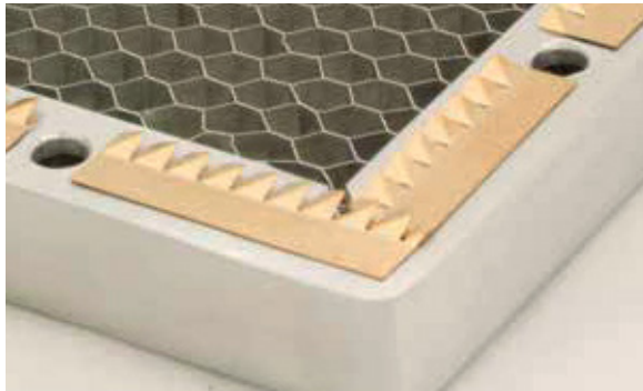
BERYLLIUM COPPER GASKET
