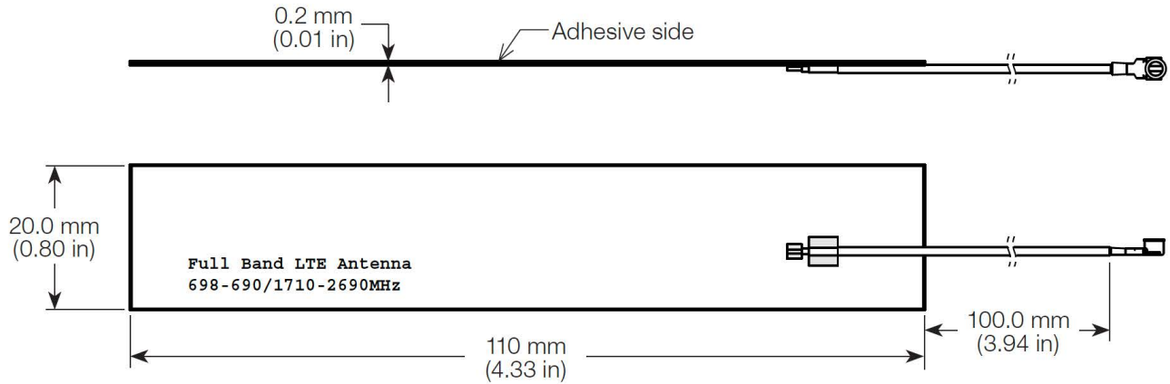
Figure 6. ANT-LPL-FPC-100 Dimensions
