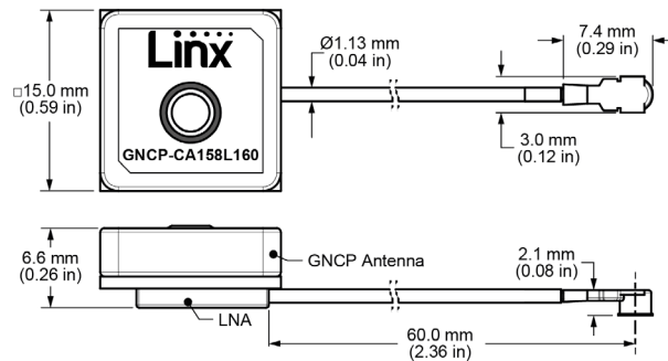
Figure 6. ANT-GNCP-CA158L160 Antenna Dimensions
