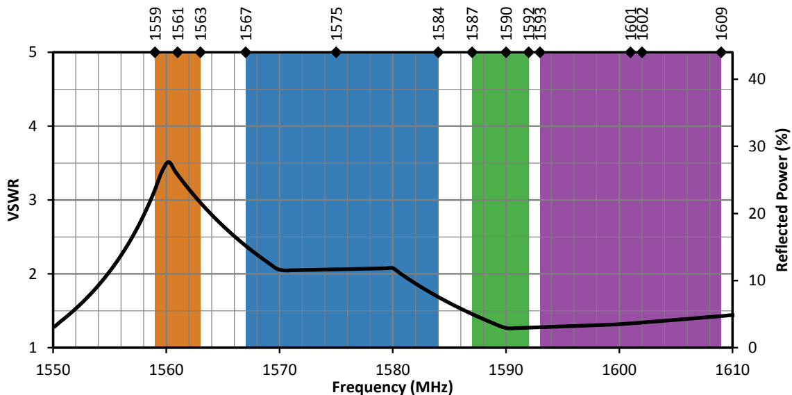
Figure 1. ANT-GNCP-CA158L160 VSWR with Frequency Band Highlights
