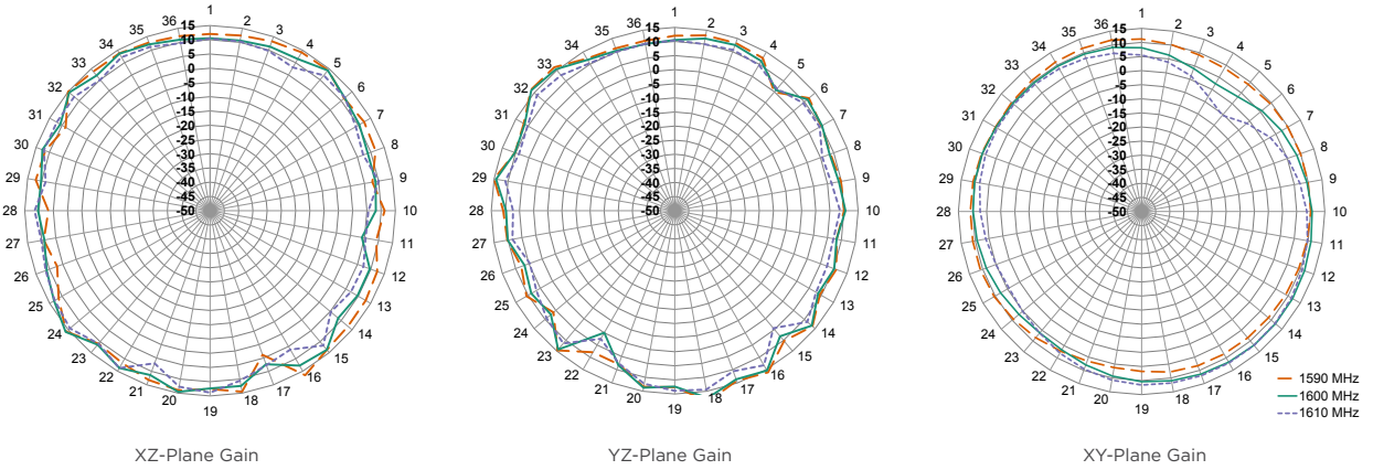
Figure 5. ANT-GNCP-CA158L160 Radiation Patterns
