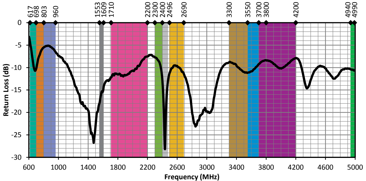
Figure 5. ANT-5GWWS2-SMA Return Loss, Straight
