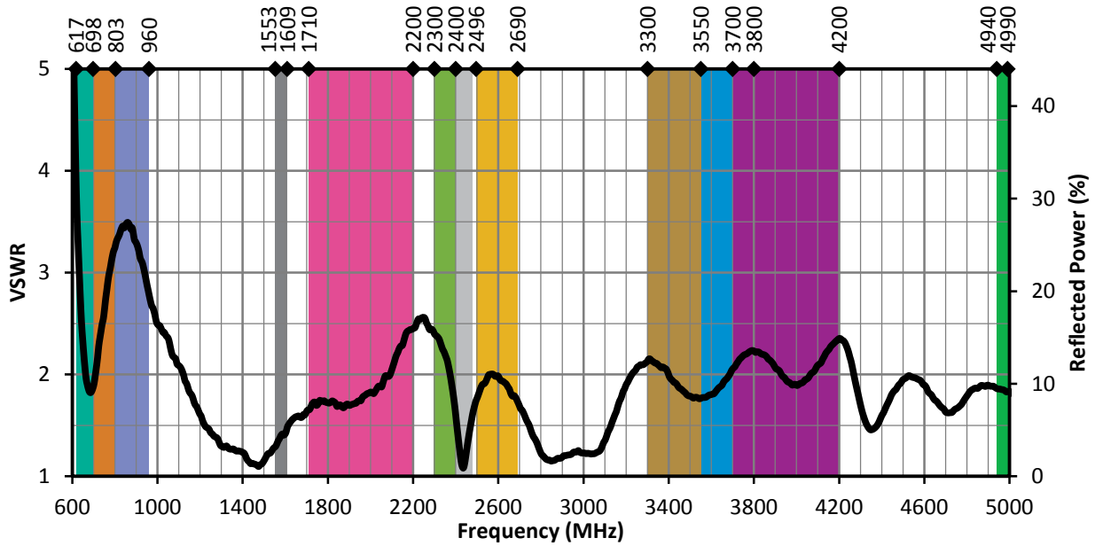
Figure 4. ANT-5GWWS2-SMA VSWR, Straight
