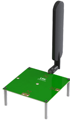
Figure 10. ANT-5GWWS2-SMA on Edge of Ground Plane, Bent 90 Degrees (Edge-Bent)
