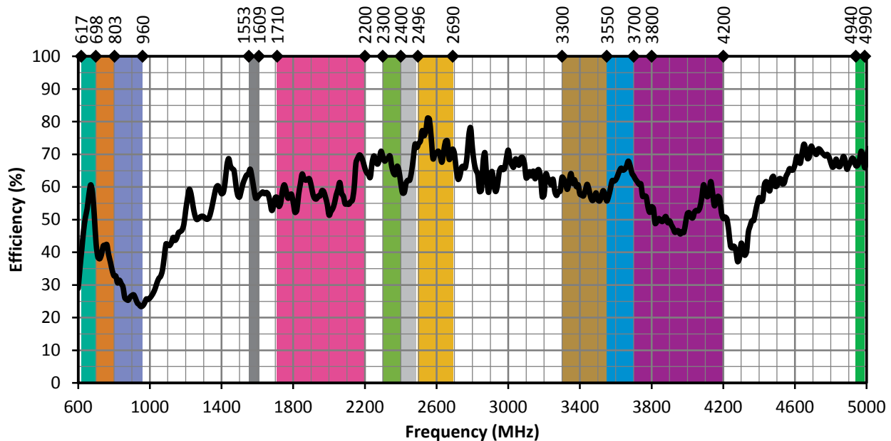
Figure 8. ANT-5GWWS2-SMA Antenna Efficiency, Straight
