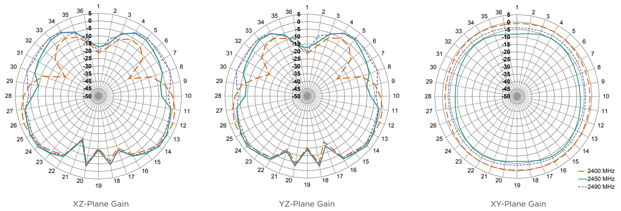
Figure 8. Radiation Patterns for ANT-5GWWS2-SMA, Straight
