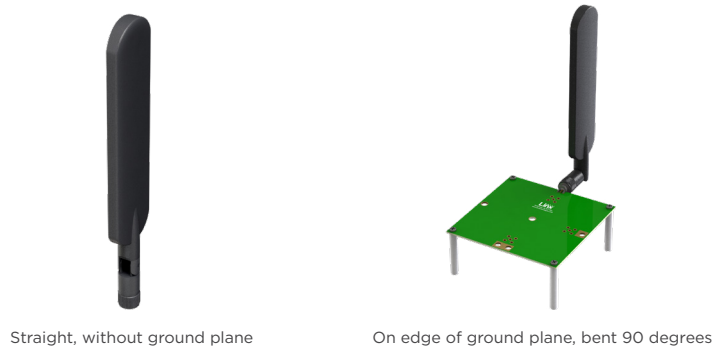
Figure 2. ANT-5GWWS2-SMA on evaluation PCB
