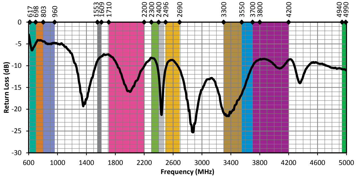
Figure 12. ANT-5GWWS2-SMA Return Loss, Edge-Bent
