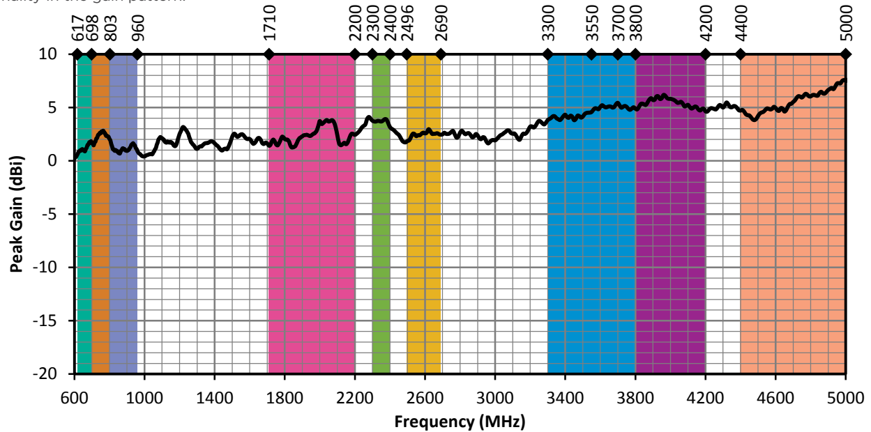
Figure 6. ANT-5GW-IPW1-NP Peak Gain, Free Space
