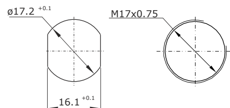
Mounting Hole
