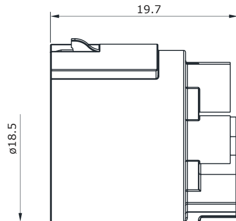
Main Dimensions insulation insert
