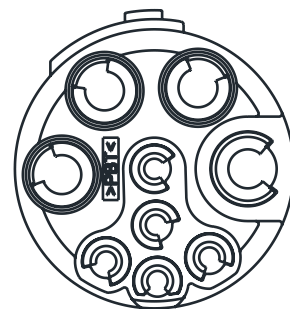
Contact Arrangement mating view
