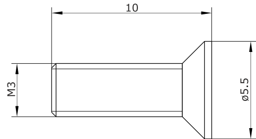
Main Dimensions screw
