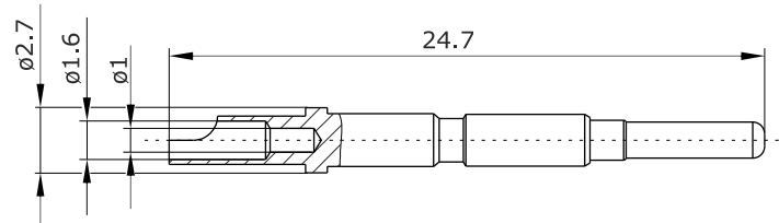
Main Dimensions contact pin
