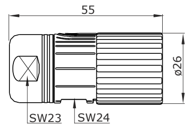
Main Dimensions plug
