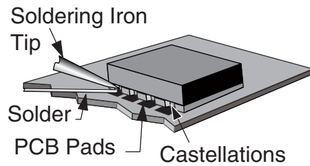
Figure 29: Soldering Technique
