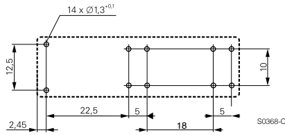
2 form A + 2 form B, 2 NO + 2 NC versions
