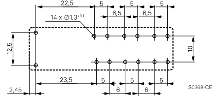
5 form A + 1 form B, 5 NO + 1 NC versions SR6
