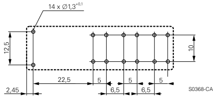
3 form A + 3 form B, 3 NO + 3 NC versions SR6
