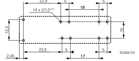
3 form A + 1 form B, 3 NO + 1 NC contacts
