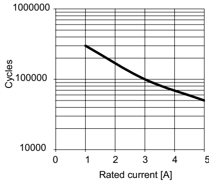
Characteristically electrical endurance acc. IEC60947-5-1 DC-1 Ue=24VDC
