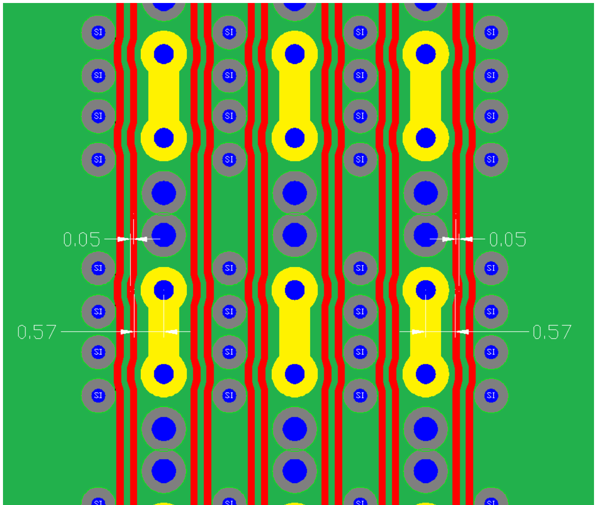
Figure 10: Daughtercard Channel Routing with 5-5-5 trace
