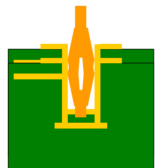
Figure 9: Blind Via
