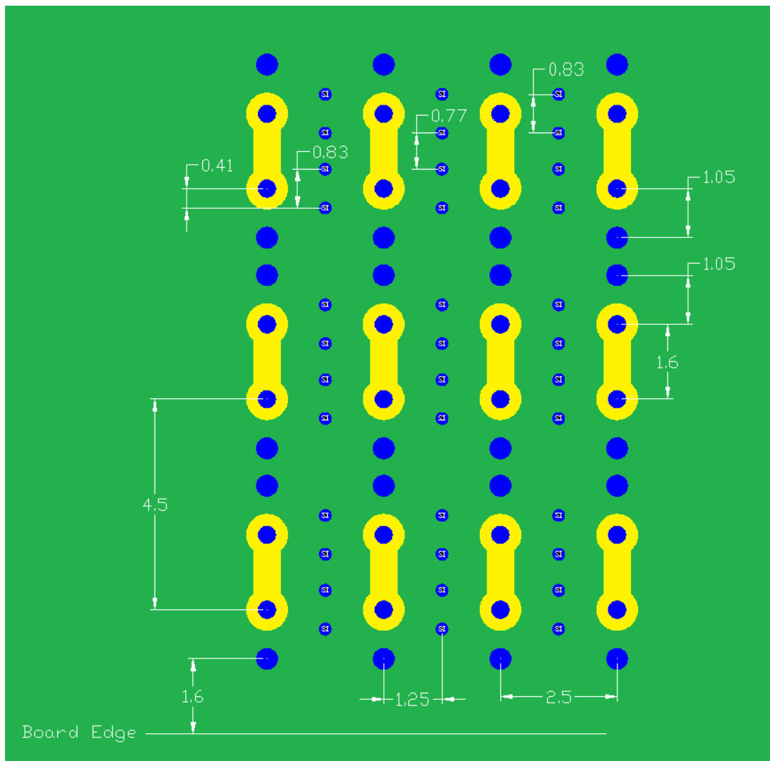
Figure 2: STRADA Whisper Daughtercard Footprint Dimensions
