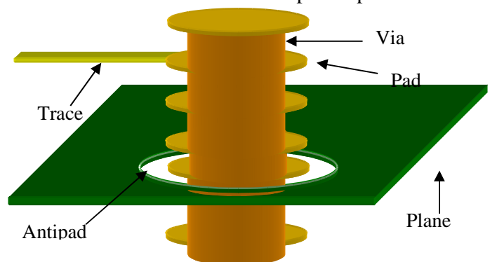
Figure 3: Antipad Illustration
