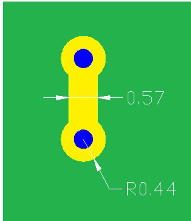
Figure 4: Daughtercard Antipad Geometry
