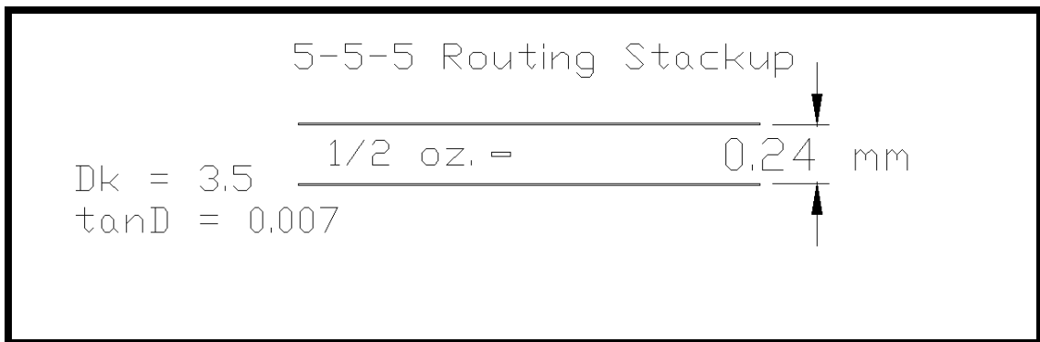
Figure 14: 5-5-5 Routing
