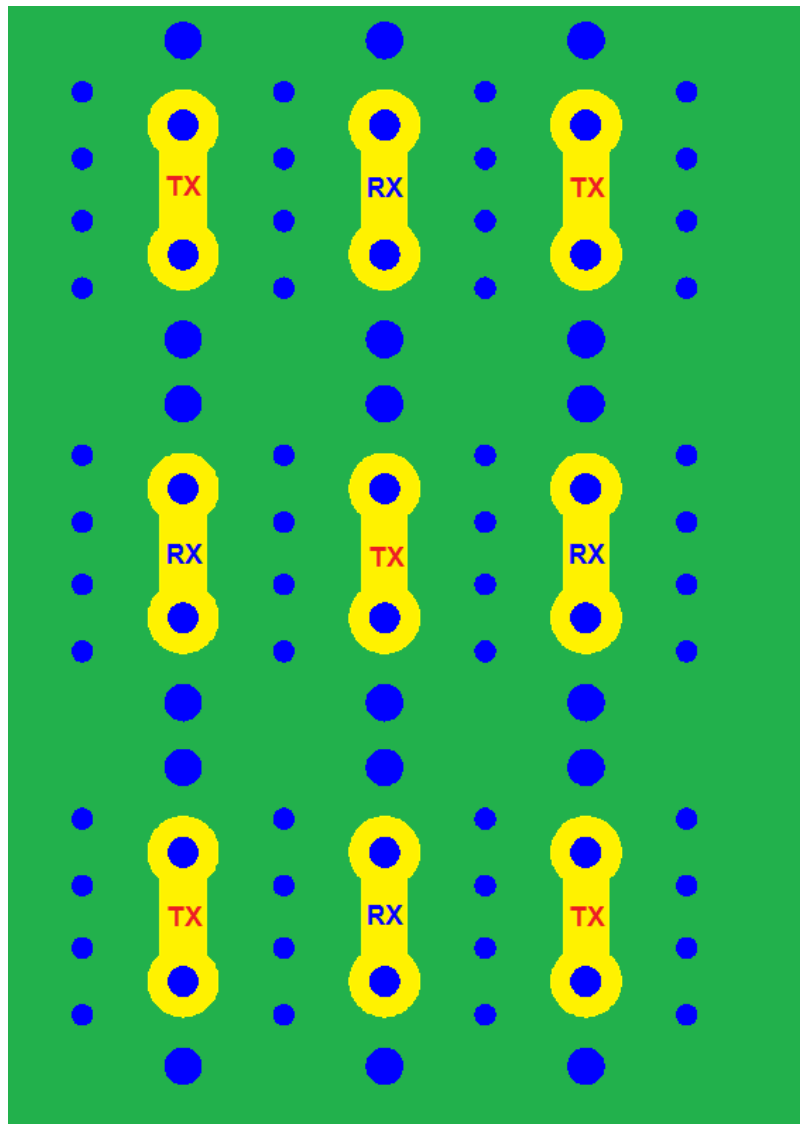
Figure 13: Interstitial Pinout
