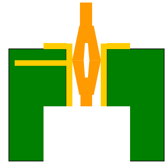
Figure 8: Counterbored Via
