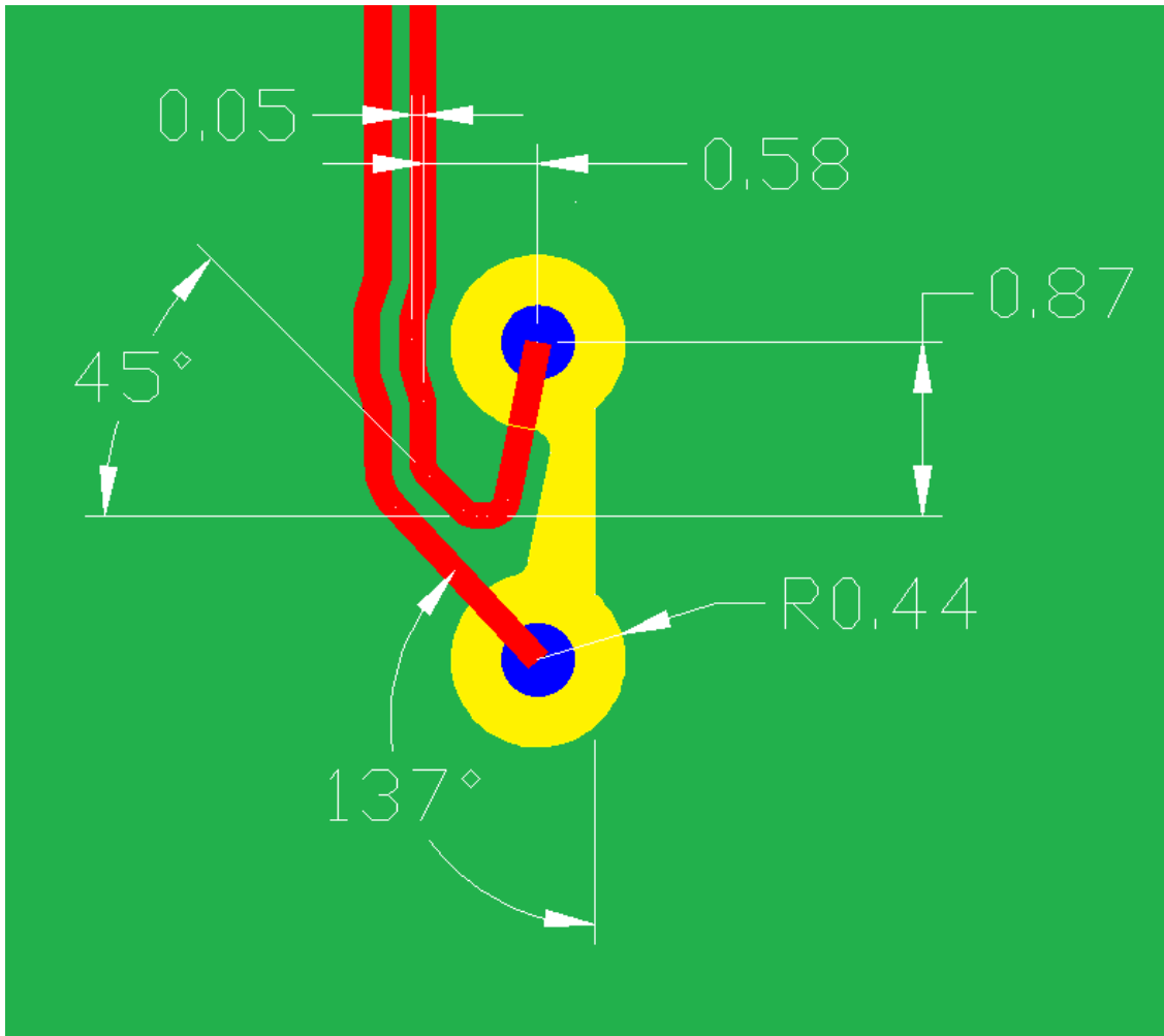
Figure 5: Daughtercard Breakout Antipad, Left-Side
