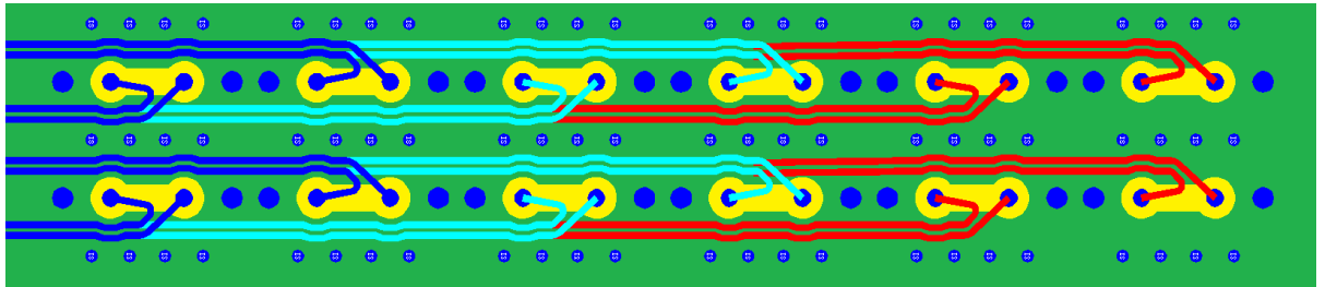
Figure 12: Typical Layer Count Breakdown for 6-pair Daughtercard Connector
