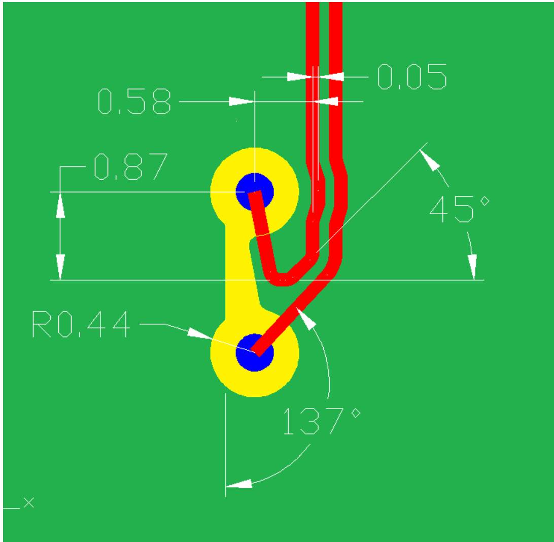
Figure 6: Daughtercard Breakout Antipad, Right-Side
