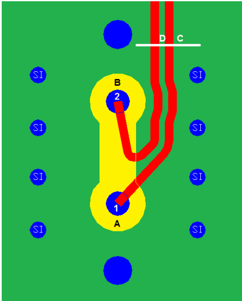
Figure 11: Example Breakout
