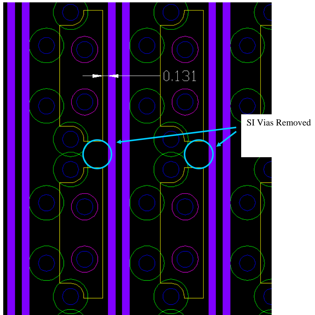
Figure 12: Alternate Backplane Routing without SI Via
