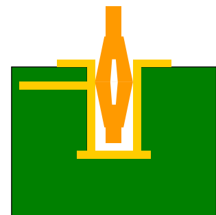
Figure 10: Blind Via
