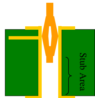
Figure 8: Via Stub
