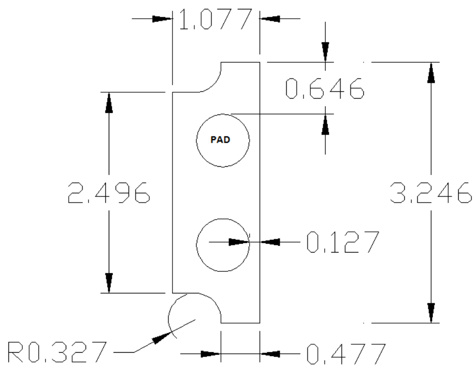
Figure 4: Backplane Antipad Geometry
