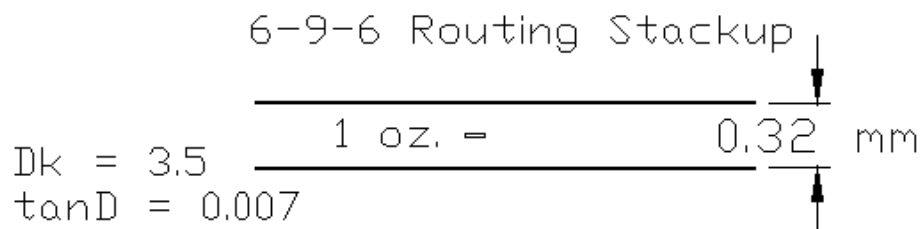
Figure 17: 6-9-6 Routing
