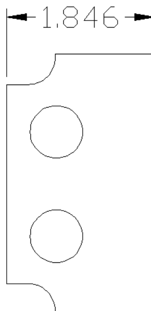
Figure 5: Alternate Backplane Antipad Geometry
