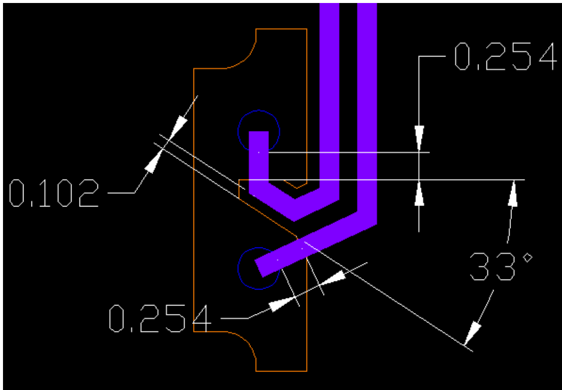
Figure 7: Backplane Breakout Antipad, Right-Side
