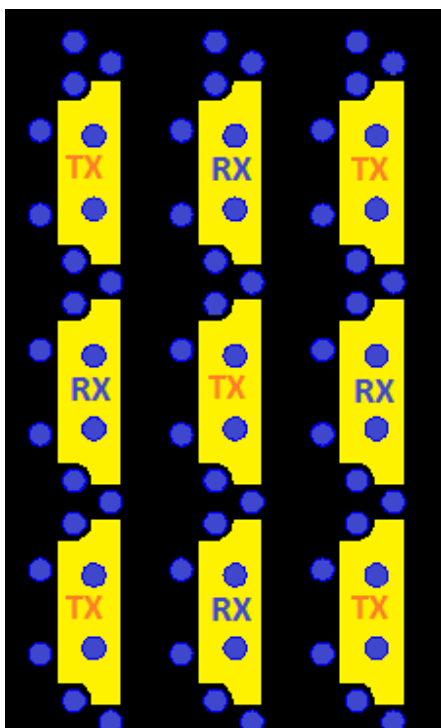
Figure 15: Interstitial Pinout
