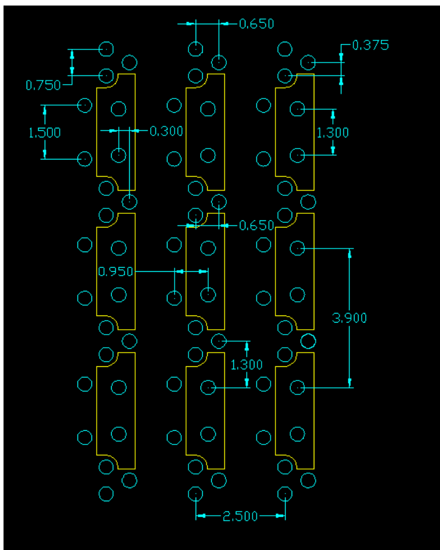
Figure 2: STRADA Whisper Backplane Footprint Dimensions
