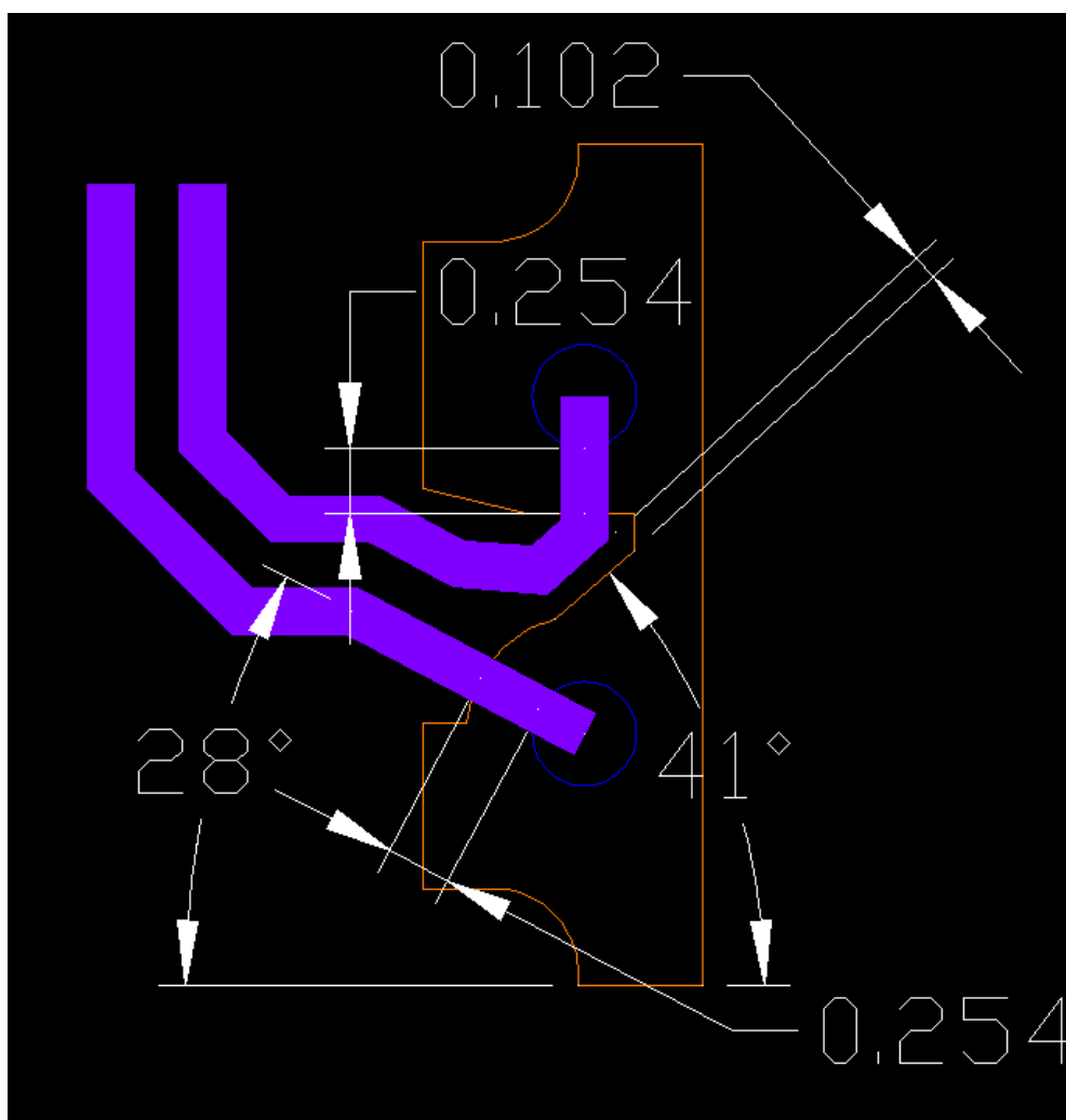
Figure 6: Backplane Breakout Antipad, Left-Side
