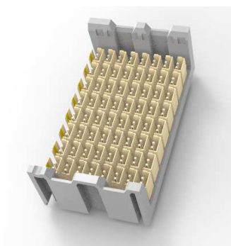
Figure 1: STRADA Whisper Pair-In-Column Connector
