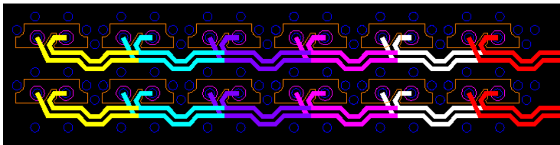
Figure 14: Typical Layer Count Breakdown for 6-pair Backplane Connector
