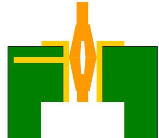
Figure 9: Counterbored Via
