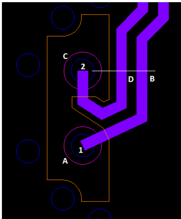
Figure 13: Example Breakout
