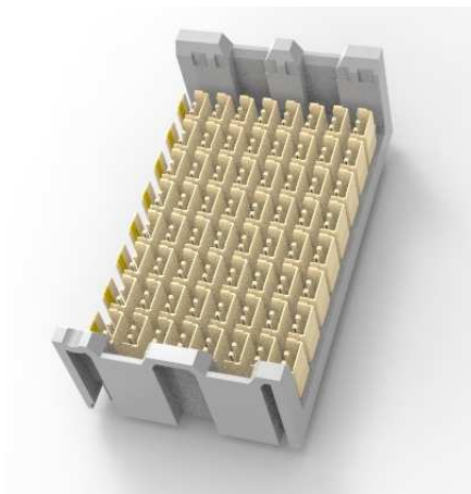
STRADA Whisper 3.9mm Pair-In-Column Connector
