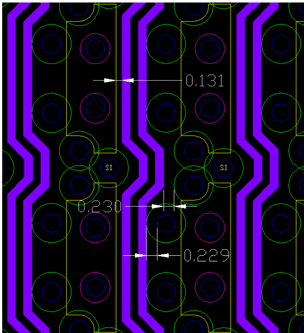
Figure 11: Backplane Channel Routing with 7-7-7 trace
