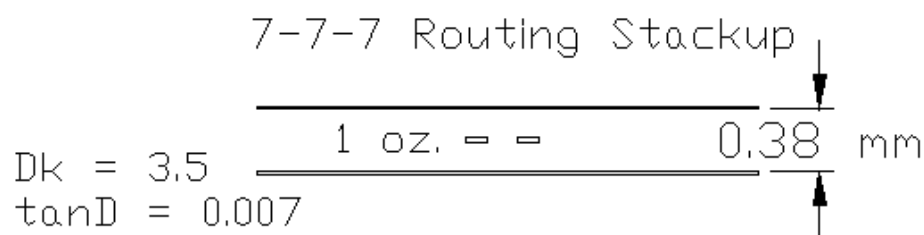
Figure 16: 7-7-7 Routing
