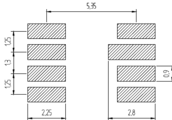
Figure 21: MS5803-07BA recommended pad layout
