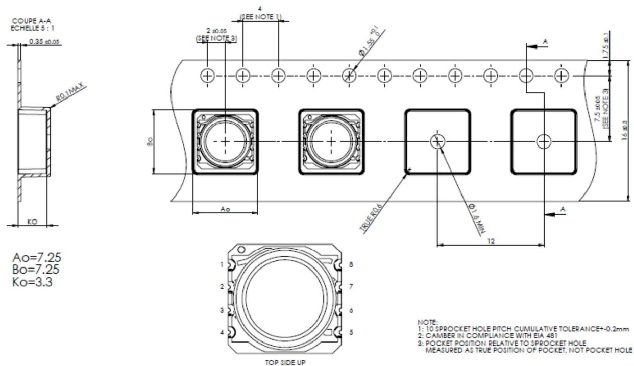
Figure 23: MS5803-07BA Tape & reel shipping package
