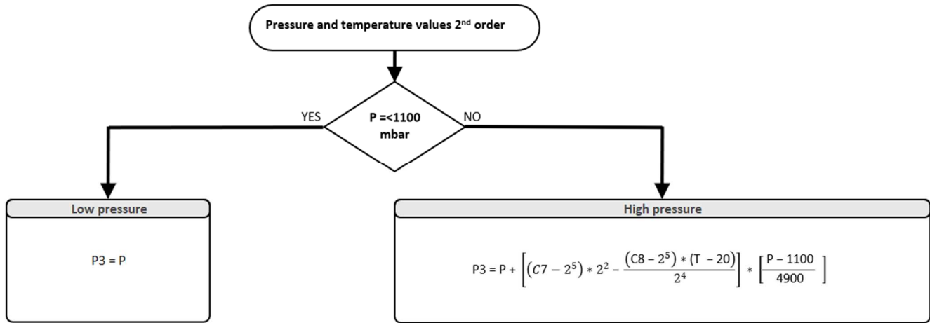
Figure 18: Flow chart for High pressure P3 calculation
