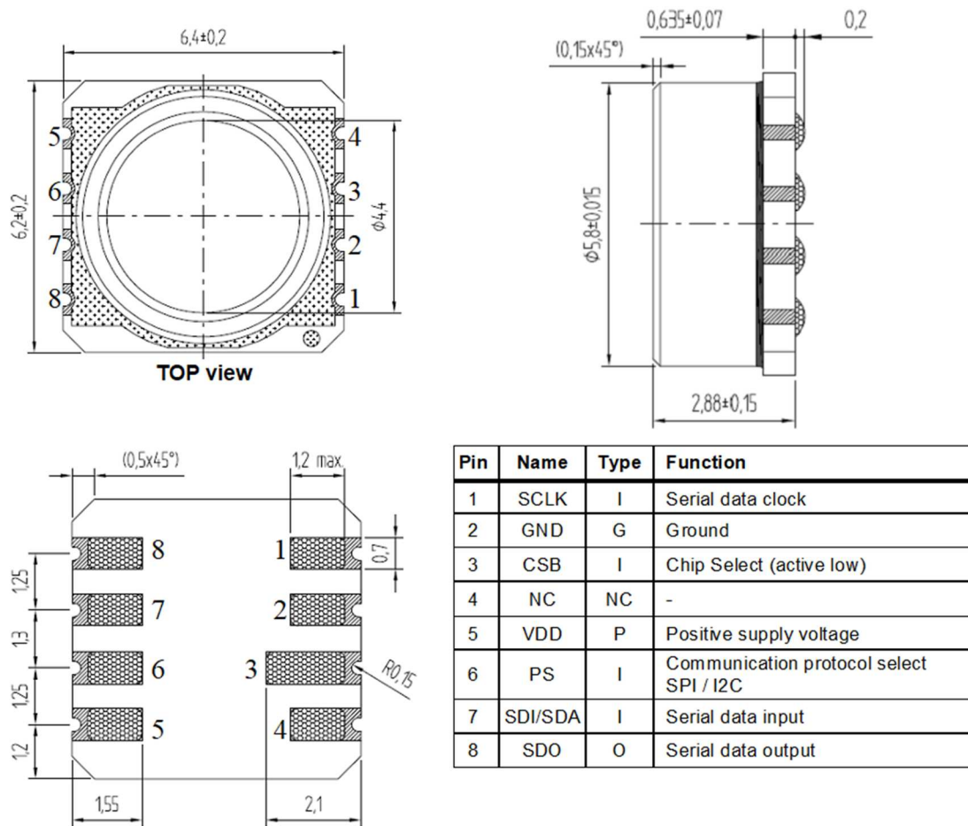
Figure 20: MS5803-07BA package outlines, pin configuration and description
