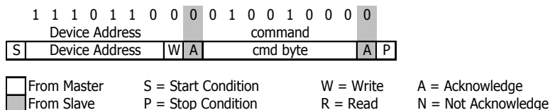
Figure 8: I 2 C command to initiate a pressure conversion (OSR=4096, typ=D1)
