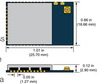
Figure 1: Package Dimensions
