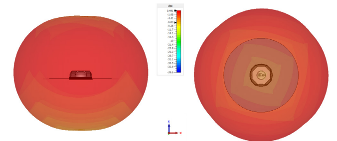
Radiation Patterns at 960 MHz
