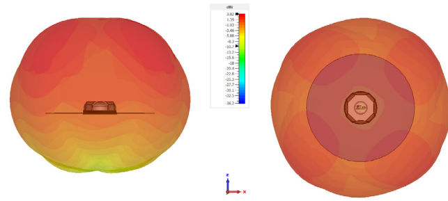
Radiation Patterns at 2170 MHz
