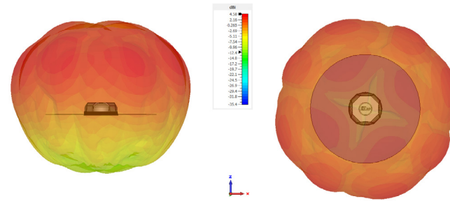
Radiation Patterns at 2700 MHz
