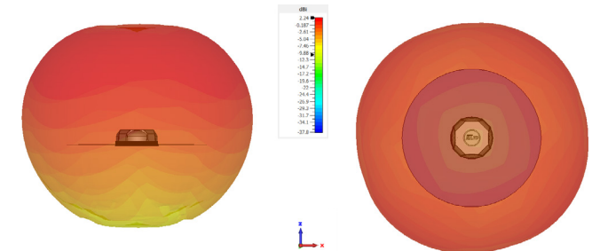
Radiation Patterns at 1690 MHz
