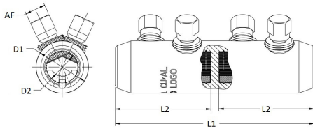
Mechanical Connector
