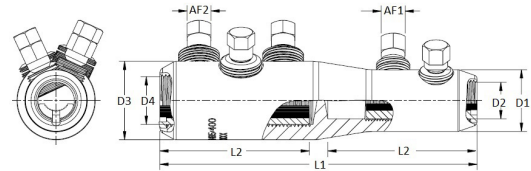
Reduction Connector
