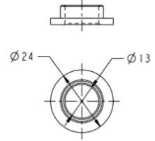
Reducing bush - BLM-REDUCER-13/17
