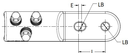
Lug with 2-holes palm
