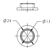
Reducing bush - BLM-REDUCER-13/17
