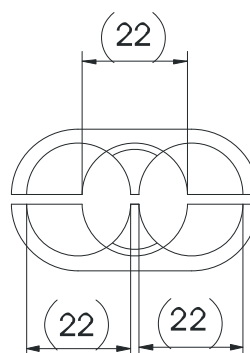
Cable Entry
