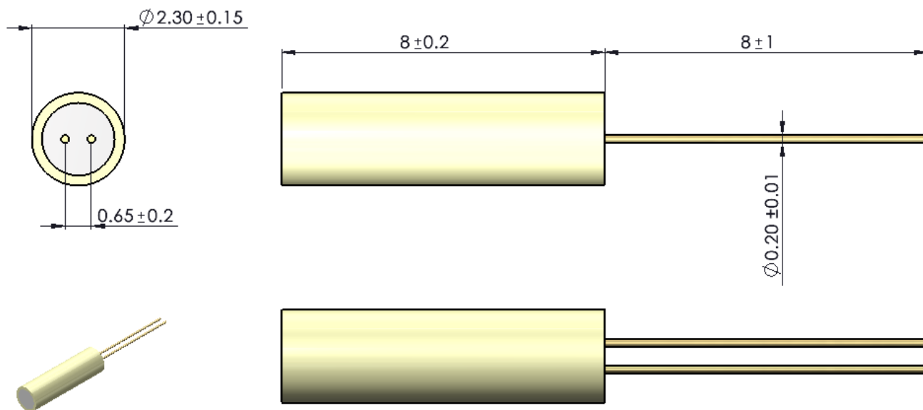
Figure 1: Mechanical dimensions of Platinum Temperature Sensor
