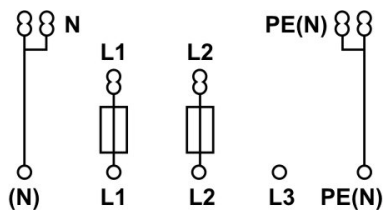
Cable entry
