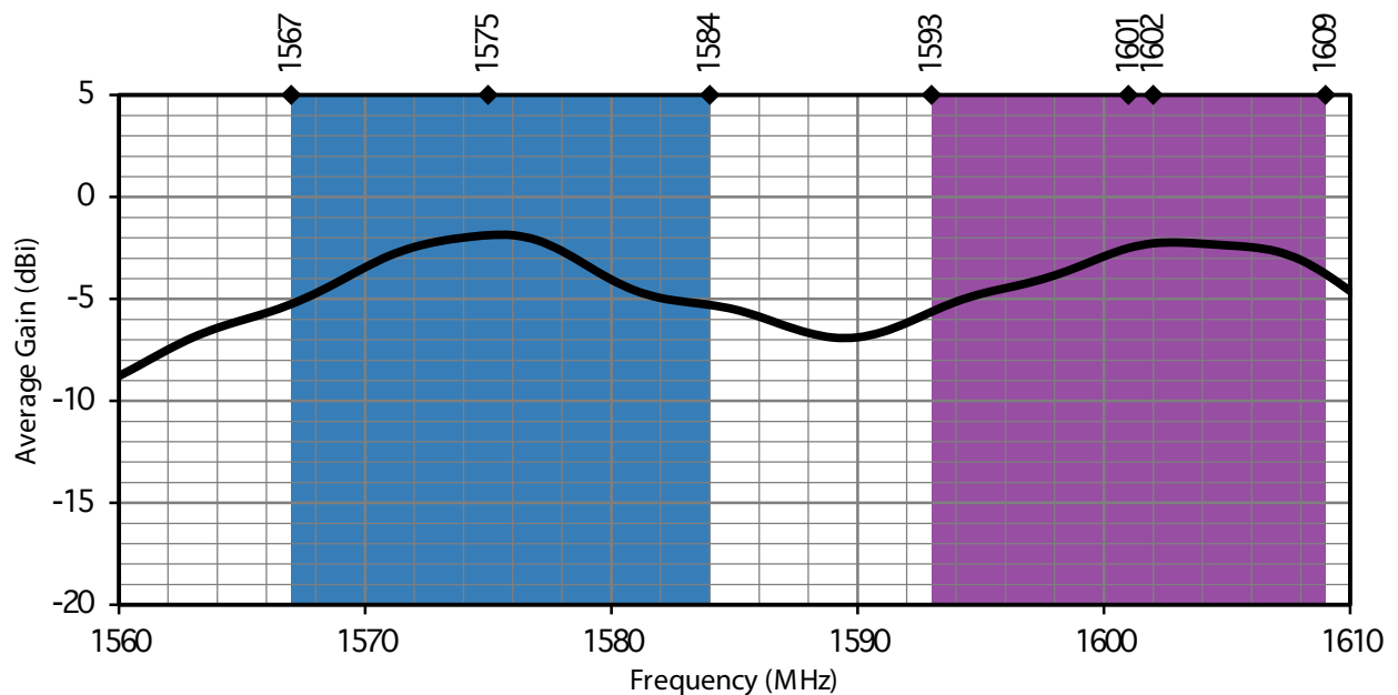
Figure 5. GNSSCP-SM12L1 Antenna Average Gain
