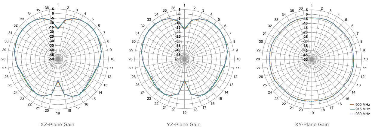
Figure 16. Radiation Patterns for ANT-8/9-IPW2-NP Antenna, Center of Ground Plane
