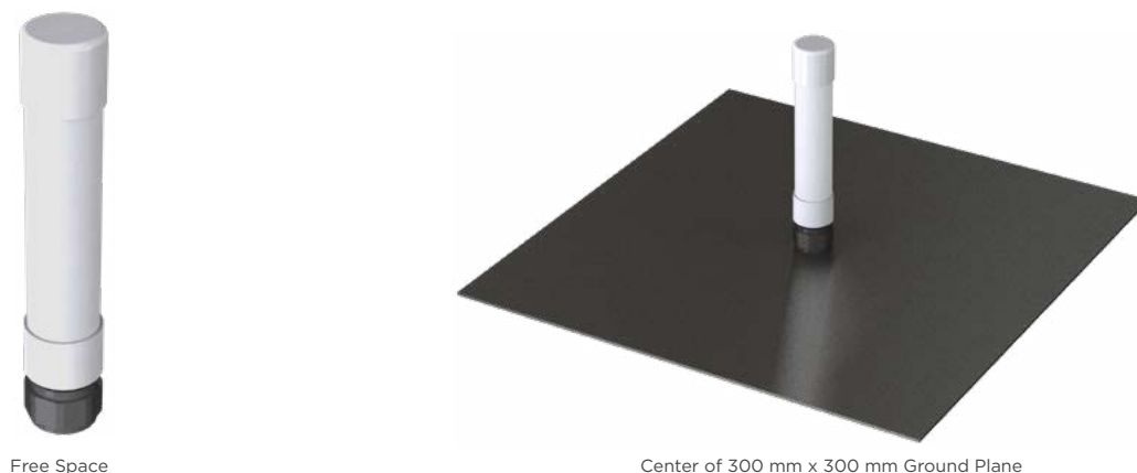
Figure 2. ANT-8/9-IPW2-NP Test Orientations
