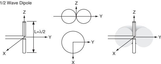
1/2 Wave Dipole
