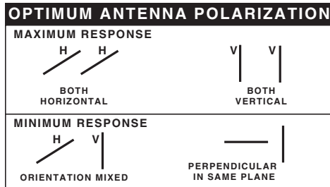
Figure 11: Antenna Polarization
