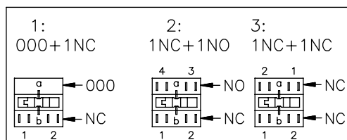
PBES16L - ILLUMINATED (WITH OR WITHOUT LAMP)
