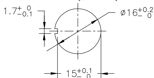
MOUNTING HOLE PBES16L - ILLUMINATED (WITH OR WITHOUT LAMP)
