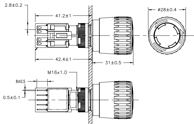
PBES16L - ILLUMINATED (WITH OR WITHOUT LAMP)
