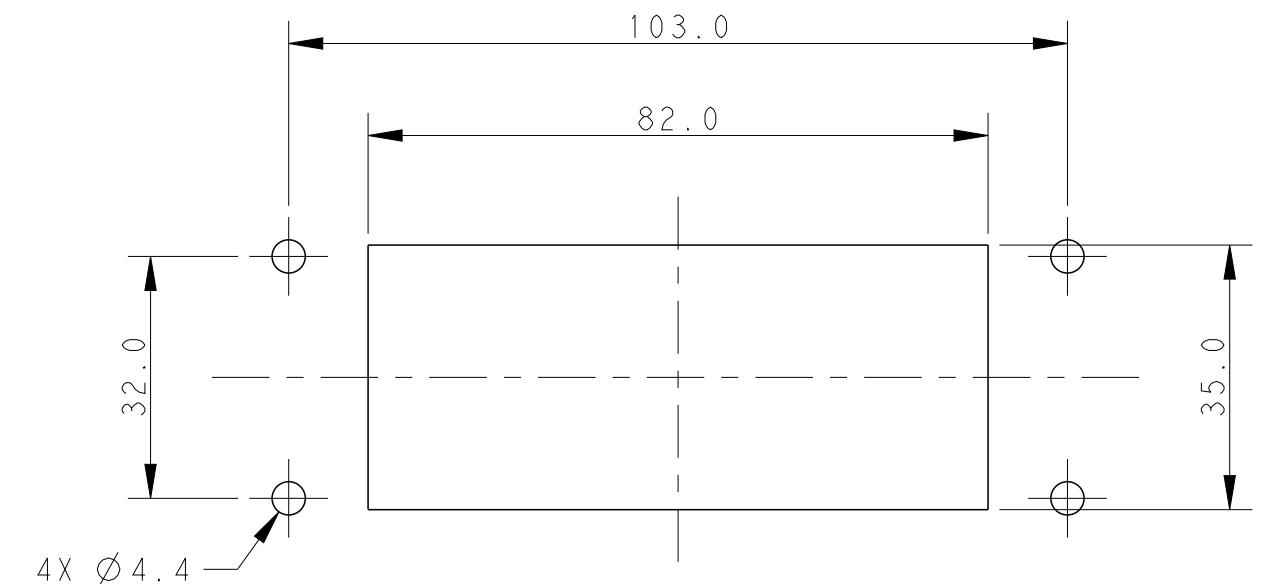
Panel Cut Out Dimension, Only for Reference 面板开口尺寸, 仅供参考
