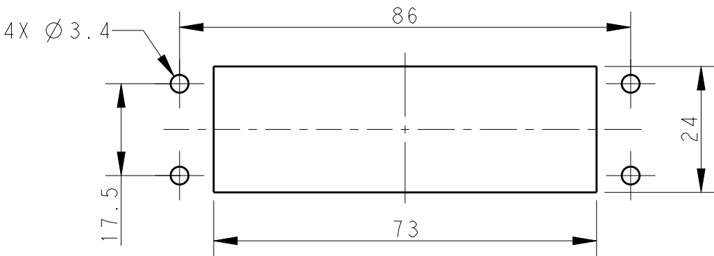
RECOMMENDED PANEL CUT OUT DIMENSIONS 推荐面板开孔尺寸
