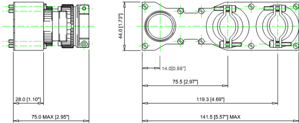
END VIEW WITH ITEM 4 CABLE CLAMP DELETED FOR CLARITY
