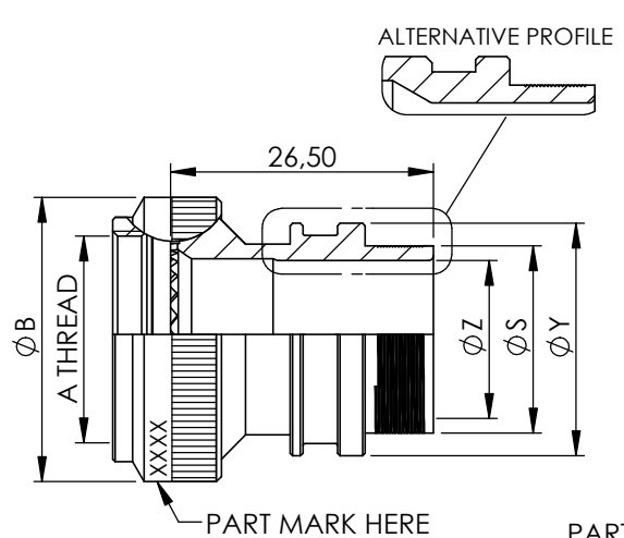
STRAIGHT BACKSHELL - TYPE 1
