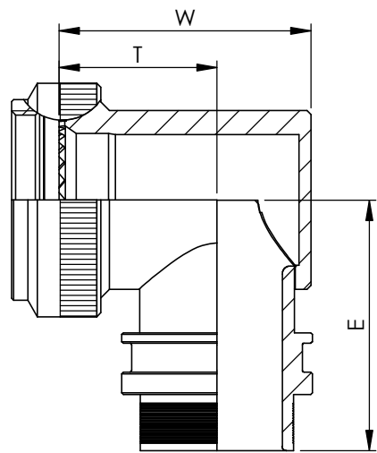
90° BACKSHELL - TYPE 1
