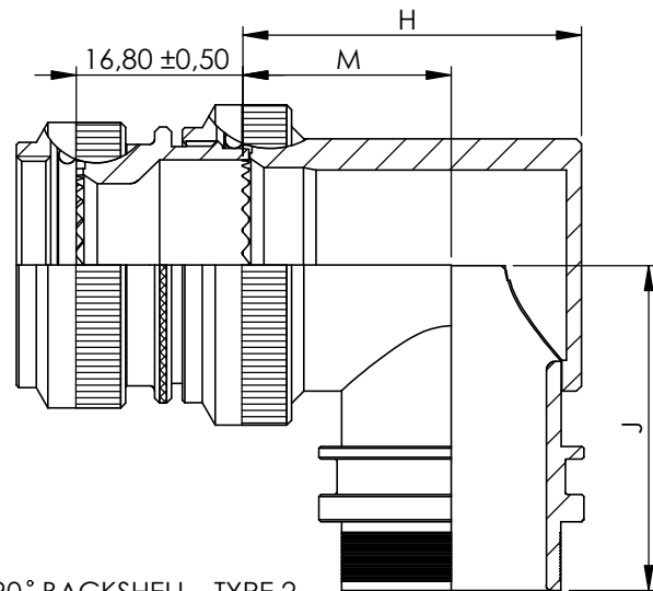
90° BACKSHELL - TYPE 2
