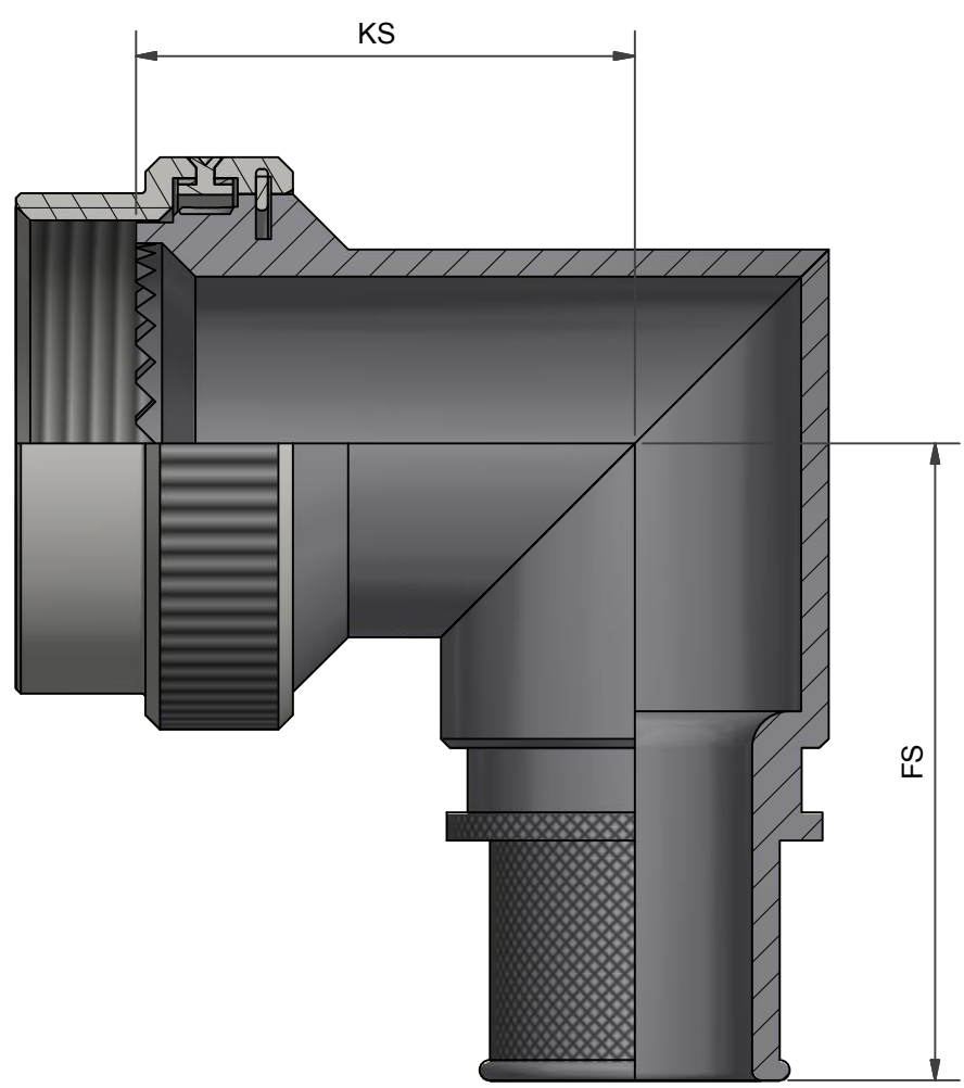
ANGLE 3 90° BACKSHELL STAINLESS STEEL NICKEL ALUMINIUM BRONZE
