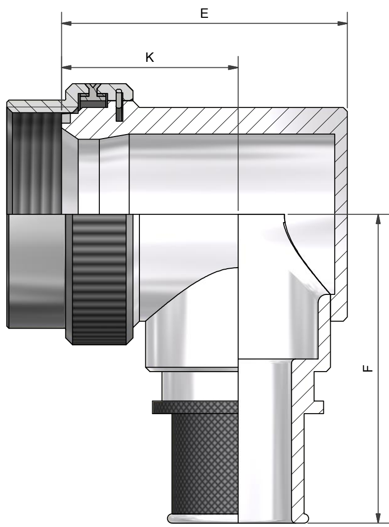
ANGLE 3 90° BACKSHELL
