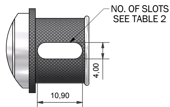
SLOT OPTION - SL (PIGTAIL TERMINATION)
