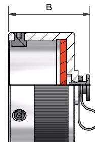
100P820S-16-1-C-EO EYELET ONLY VERSION (NO LANYARD)
