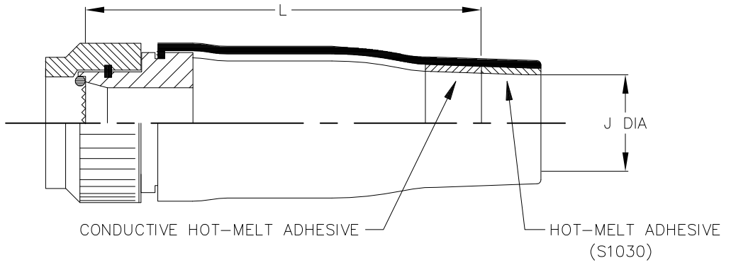
b) Part after unrestricted recovery.
