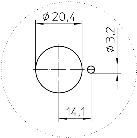
Mounting Dimensions
