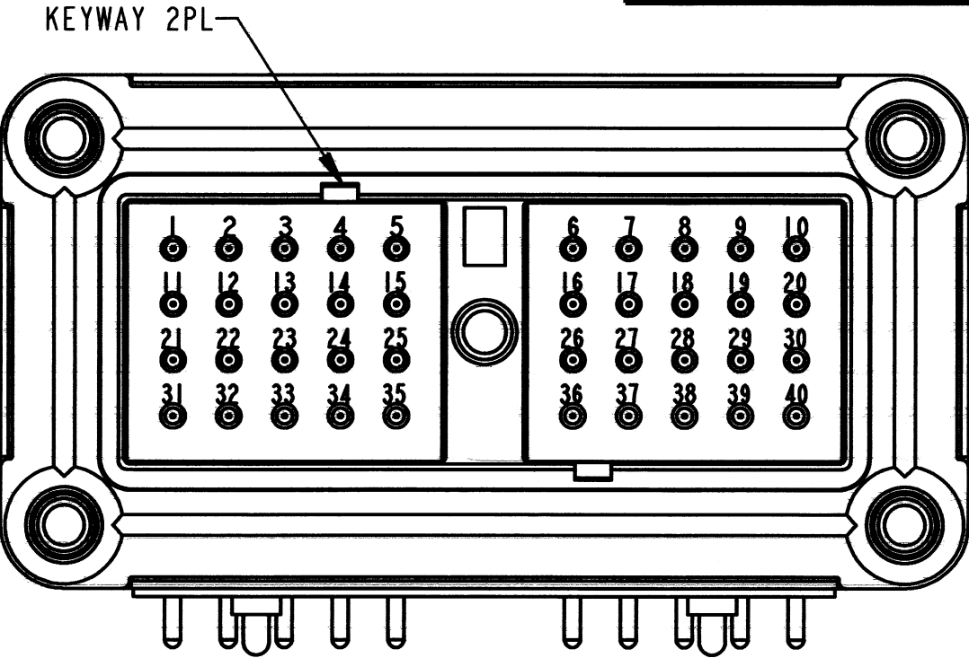
ARRANGEMENT -C- DRC13-40PC
