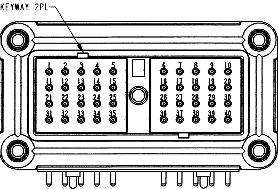
ARRANGEMENT -A- DRC13-40PA
