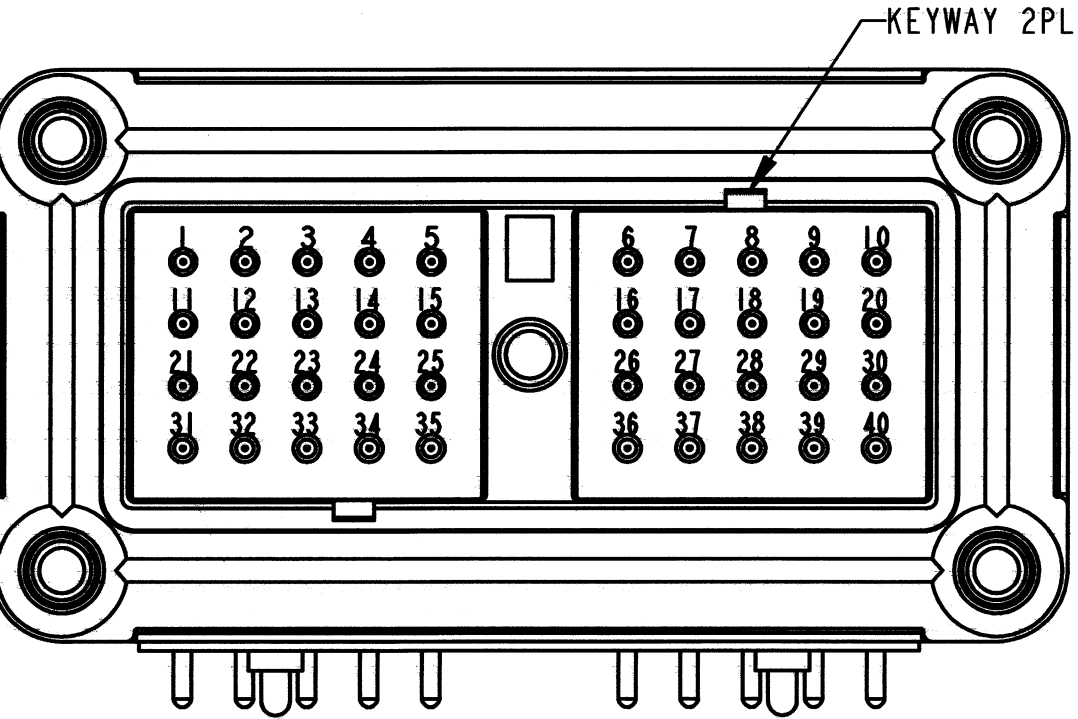
ARRANGEMENT -B- DRC13-40PB
