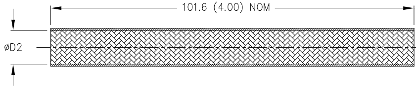
2) JUMPER BRAID
