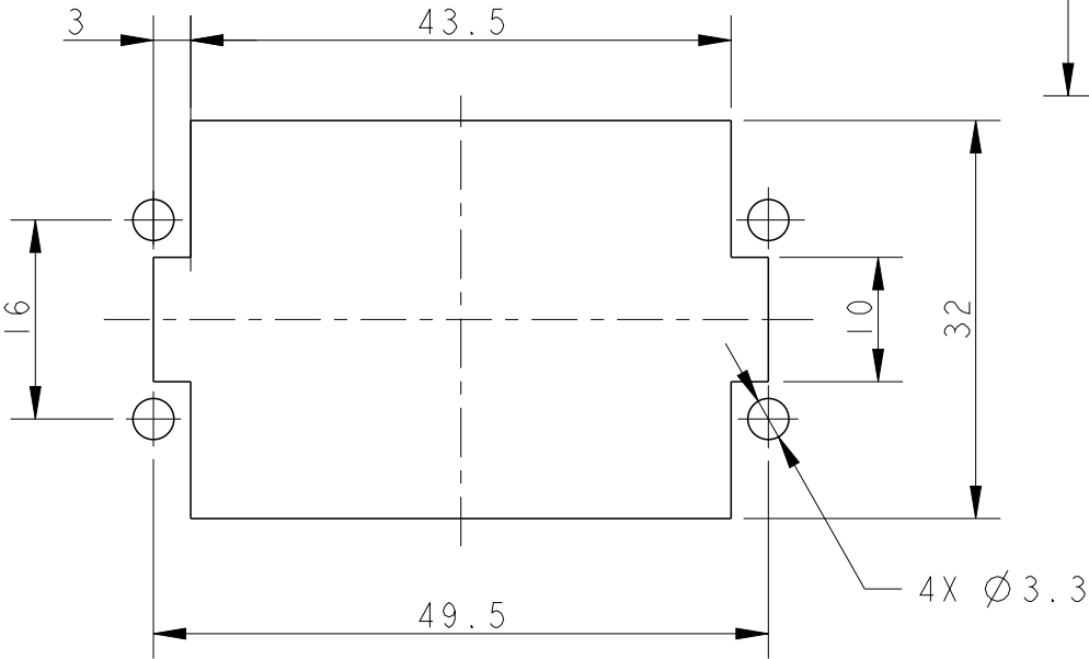
PANEL CUT FOR INSERTS FOR USING WITHOUT HOODS/ HOUSINGS 不用防护外壳时芯件的安装开孔图
