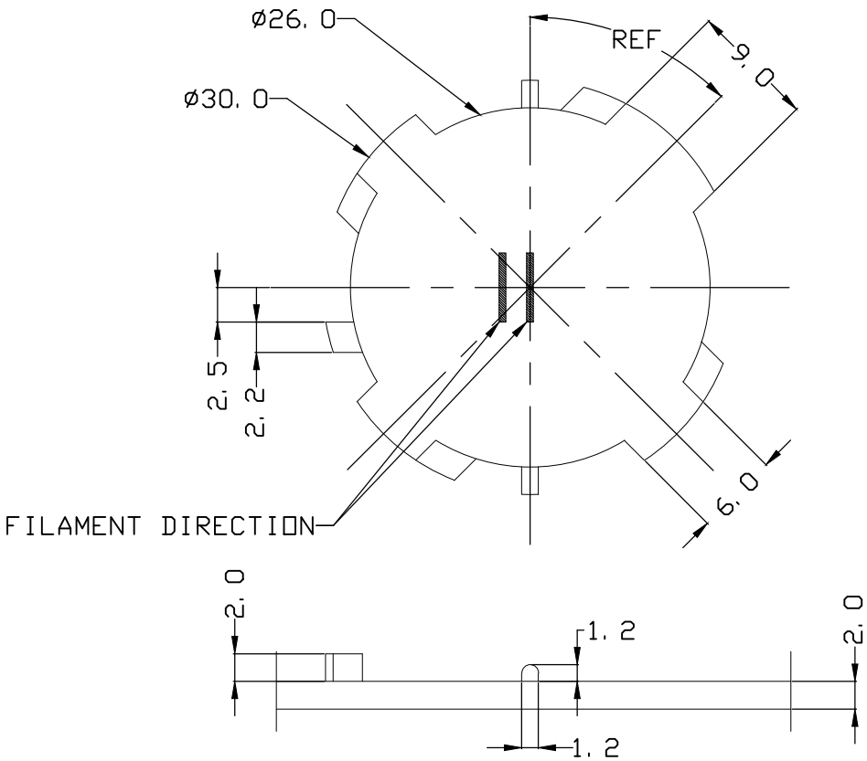
BULB POCKET LAYOUT (SCALE 2/1)
