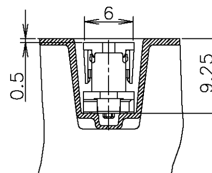
E-E (SCALE 2:1)
