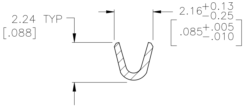
SECTION X—X
