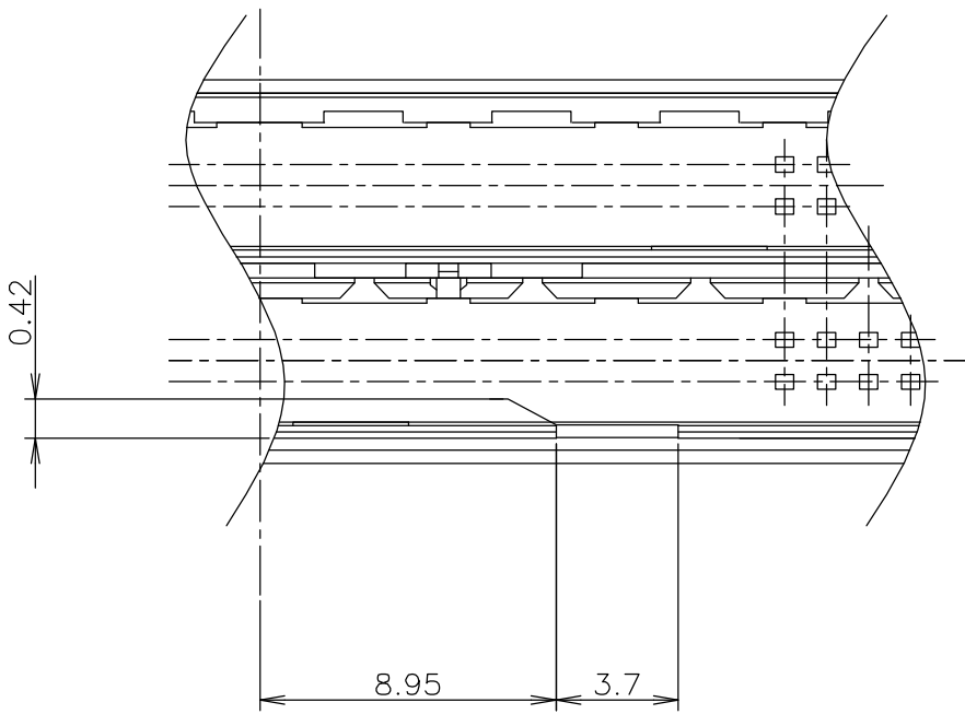
DETAIL B (SCALE 4:1) (HSG STOPPER FOR ARM BAR)
